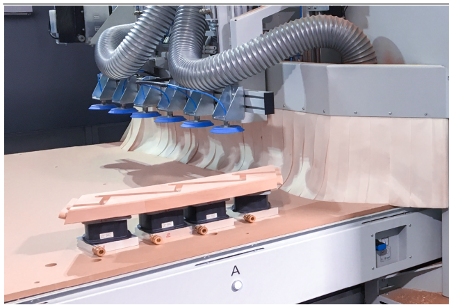
Adapter-Plates AP-G with vacuum block VCBL-B when clamping a wooden workpiece
