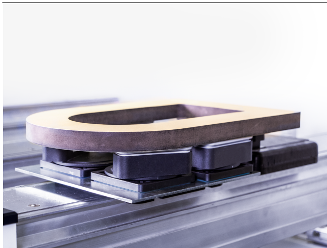
Adapter-Plates ISAP-S with Mono-Base and suction cups for clamping of curved boards
