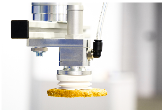
Flow gripper SCGS when handling baked goods
